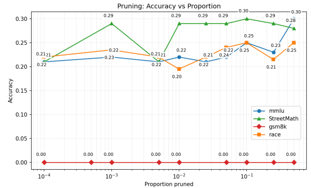
(f) Pruning accuracy on Falcon-Mamba-7B-Instruct
