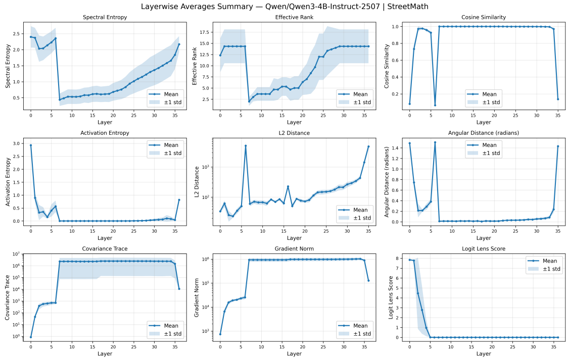
(b) Layerwise Average Summary - Qwen3-4B-Instruct-2507 on StreetMath
