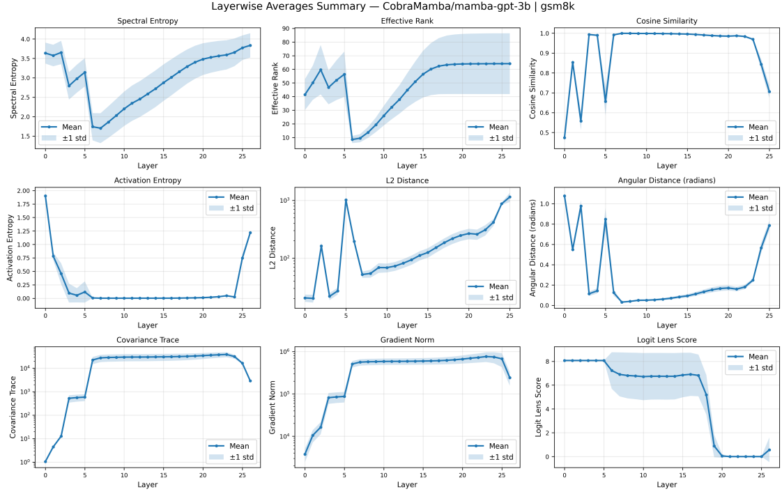
(a) Layerwise Average Summary - mamba-gpt-3B on GSM8K
