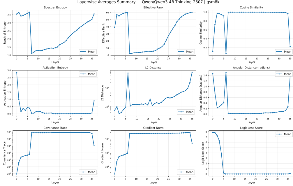
(a) Layerwise Average Summary - Qwen3-4B-Thinking-2507 on GSM8K
