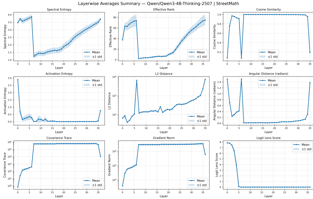
(b) Layerwise Average Summary - Qwen3-4B-Thinking-2507 on StreetMath
