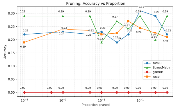
(e) Pruning accuracy on mamba-GPT-3B.png
