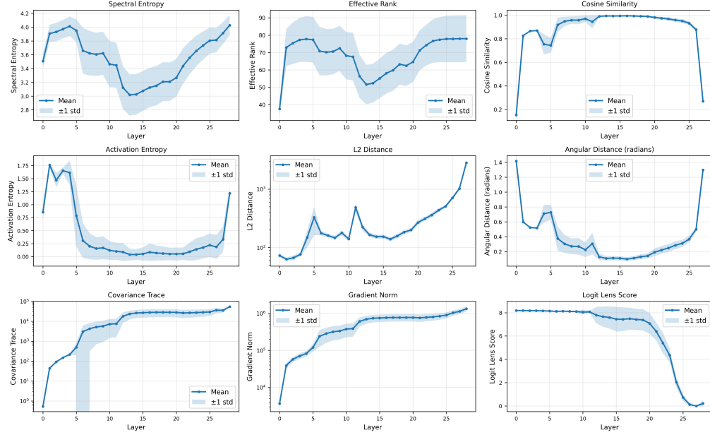
Layerwise Averages Summary — Dream-org/Dream-v0-Instruct-7B | StreetMath
