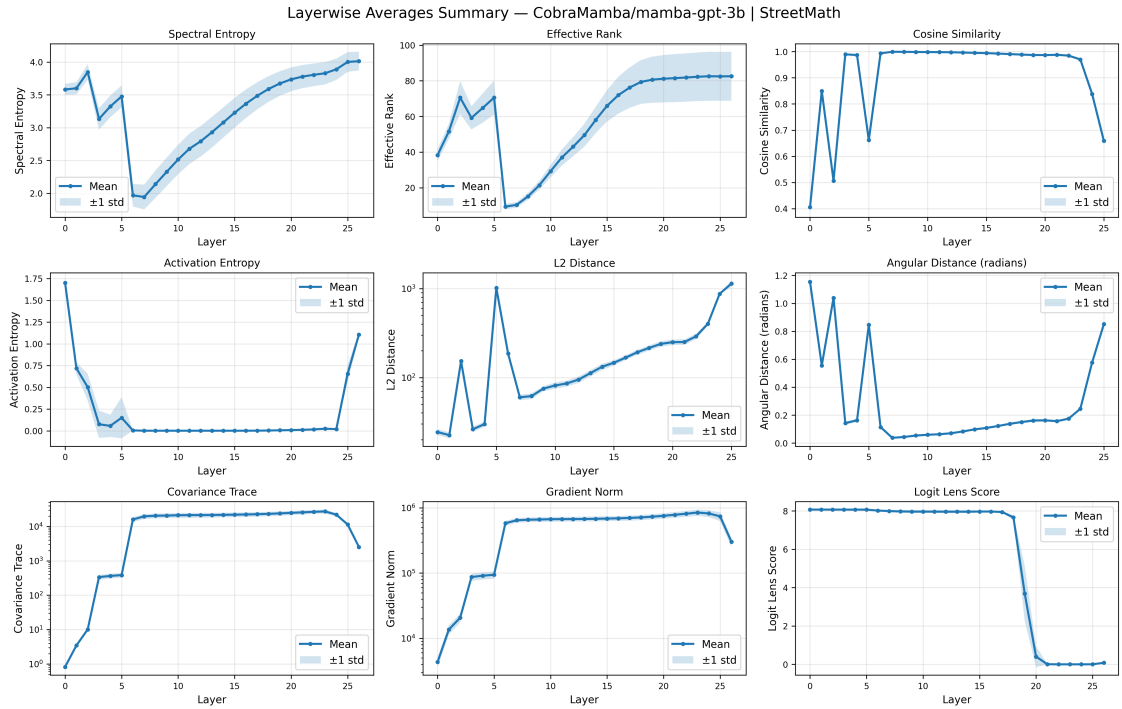
(b) Layerwise Average Summary - mamba-gpt-3B on StreetMath
