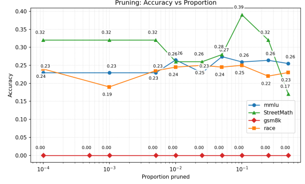
(b) Pruning accuracy on Qwen3-4B-Thinking-2507
