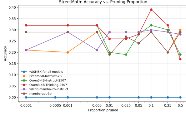
(a) Overall accuracy
