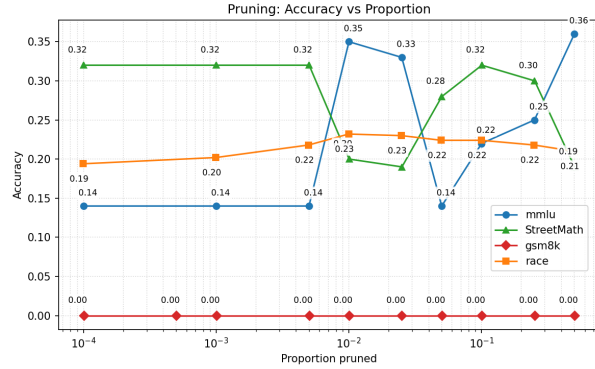
(c) Pruning accuracy on Qwen3-4B-Instruct-2507
