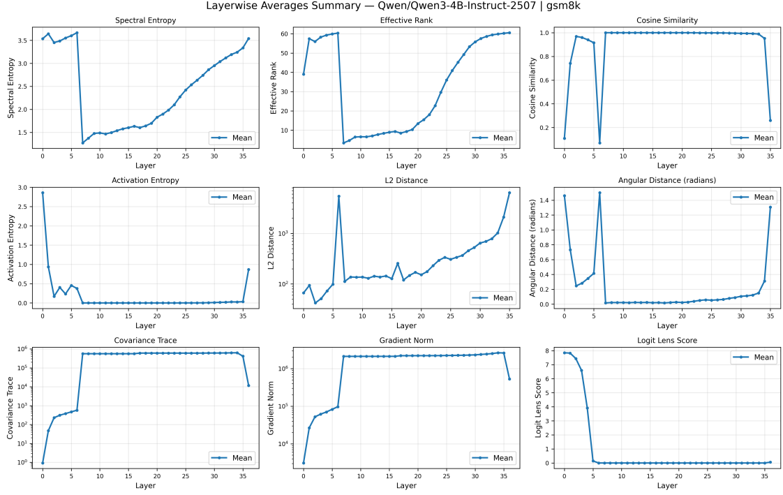
(a) Layerwise Average Summary - Qwen3-4B-Instruct-2507 on GSM8K
