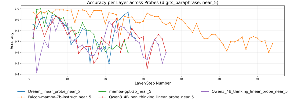
(a) Digits paraphrase (near=5)
