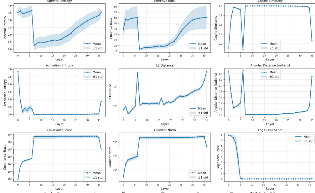
Layerwise Averages Summary — Dream-v0-Instruct-7B | gsm8k
